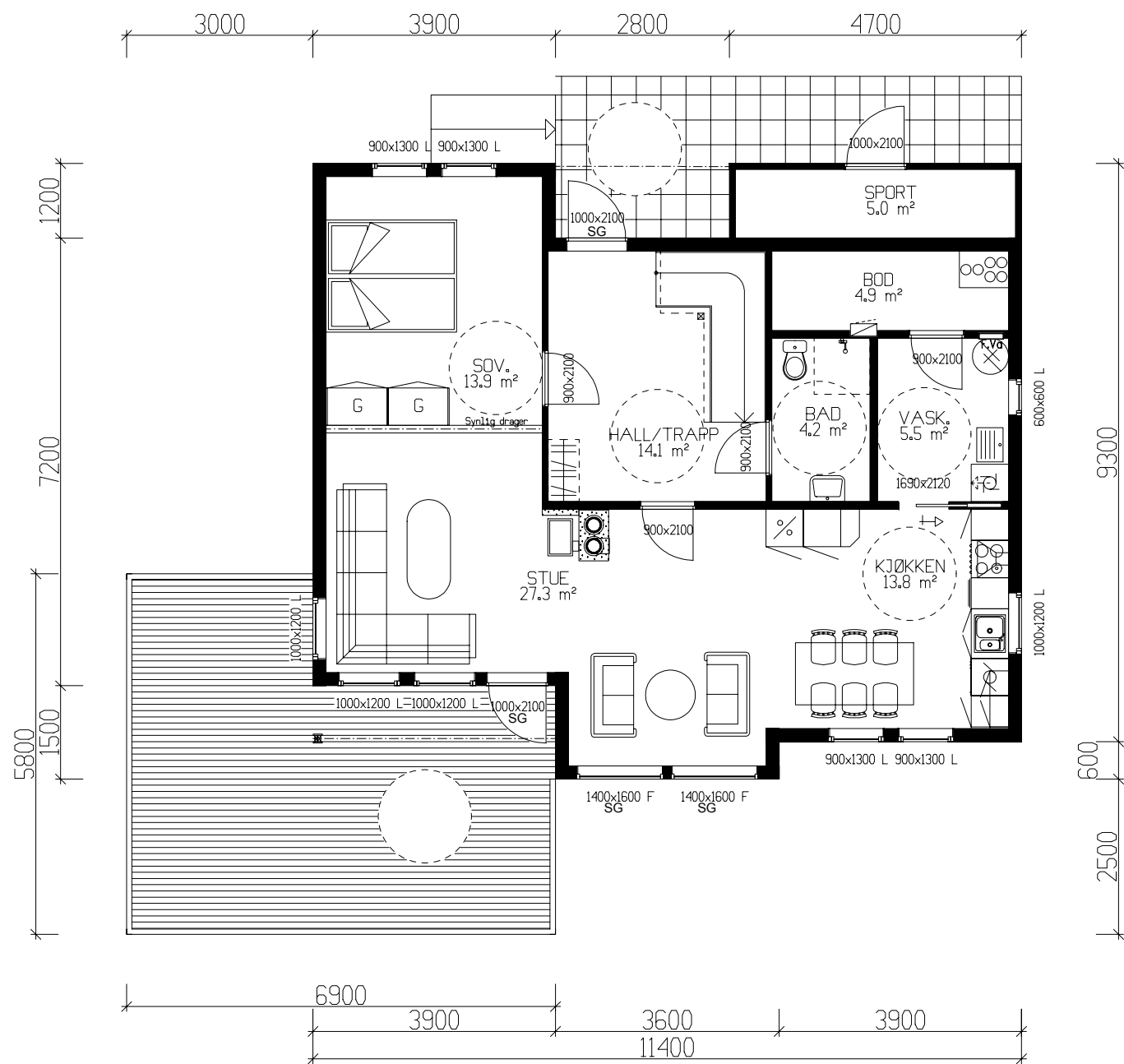
HOVEDPLAN: 86,9m² BRA + SPORT 5,0 m²
